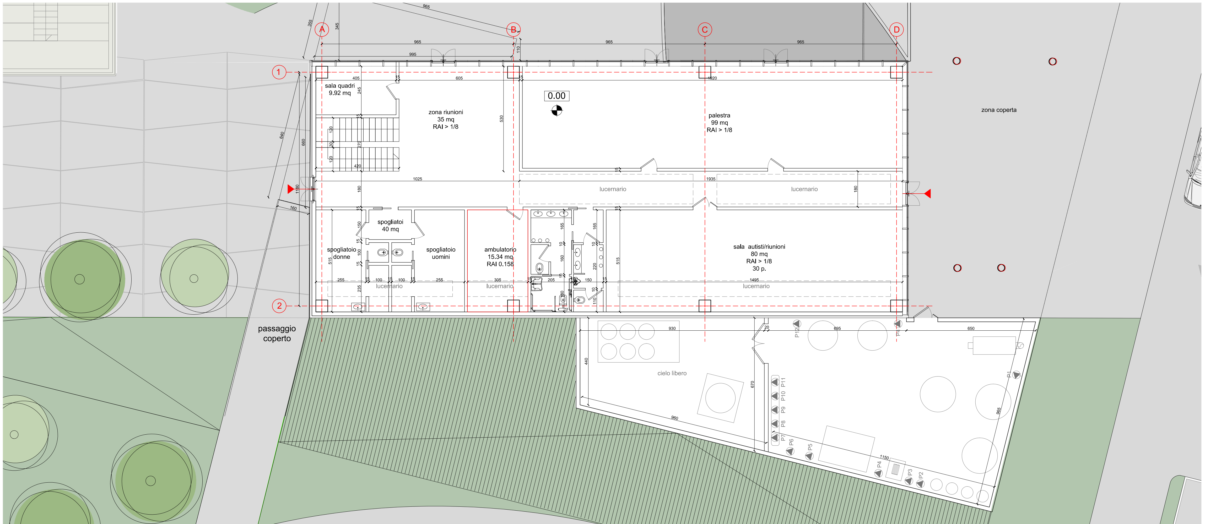
PIANO TERRA
